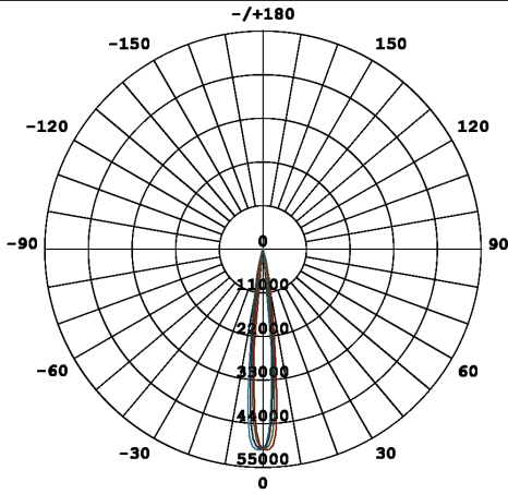
12° light distribution
