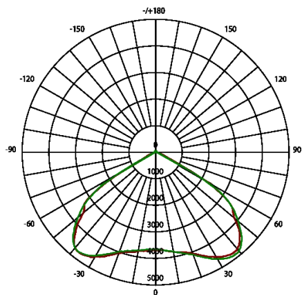
90° light distribution
