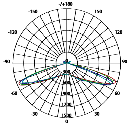
130° light distribution
